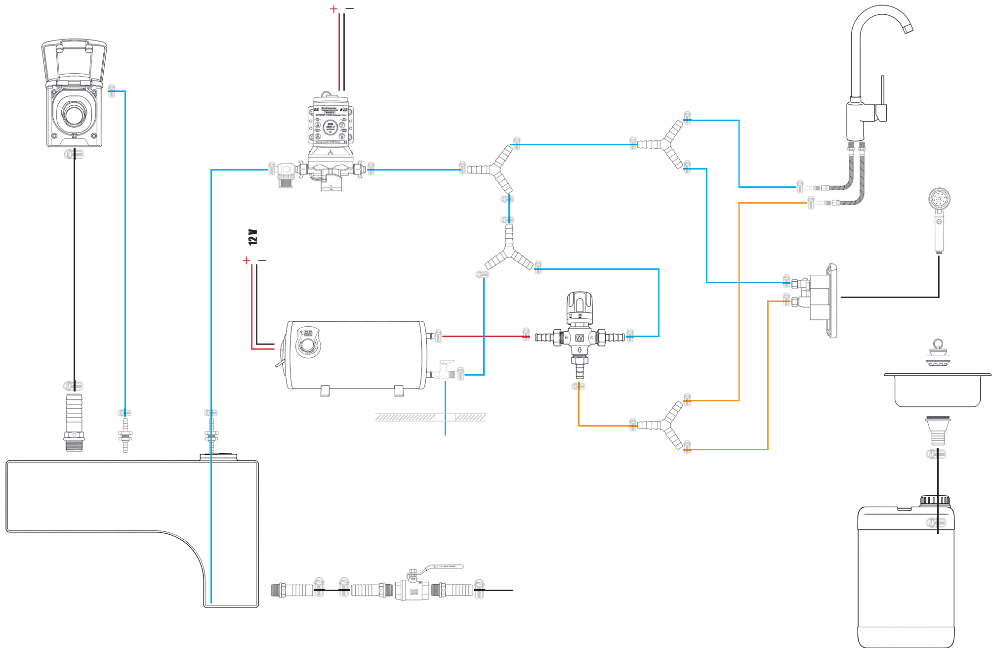
W100_Schema Wasser (Boiler, Abwasserkanister)
