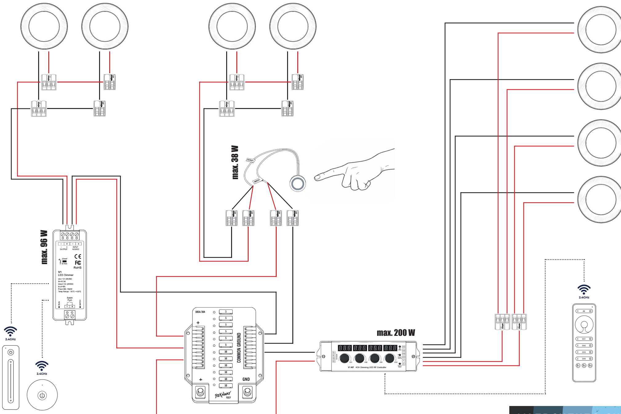
E140_Schema Elektro (Dimmer, LED)
