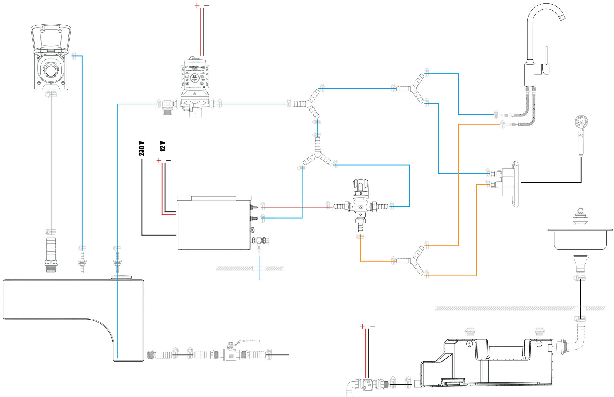
W110_Schema Wasser (Boiler, Unterflurtank)
