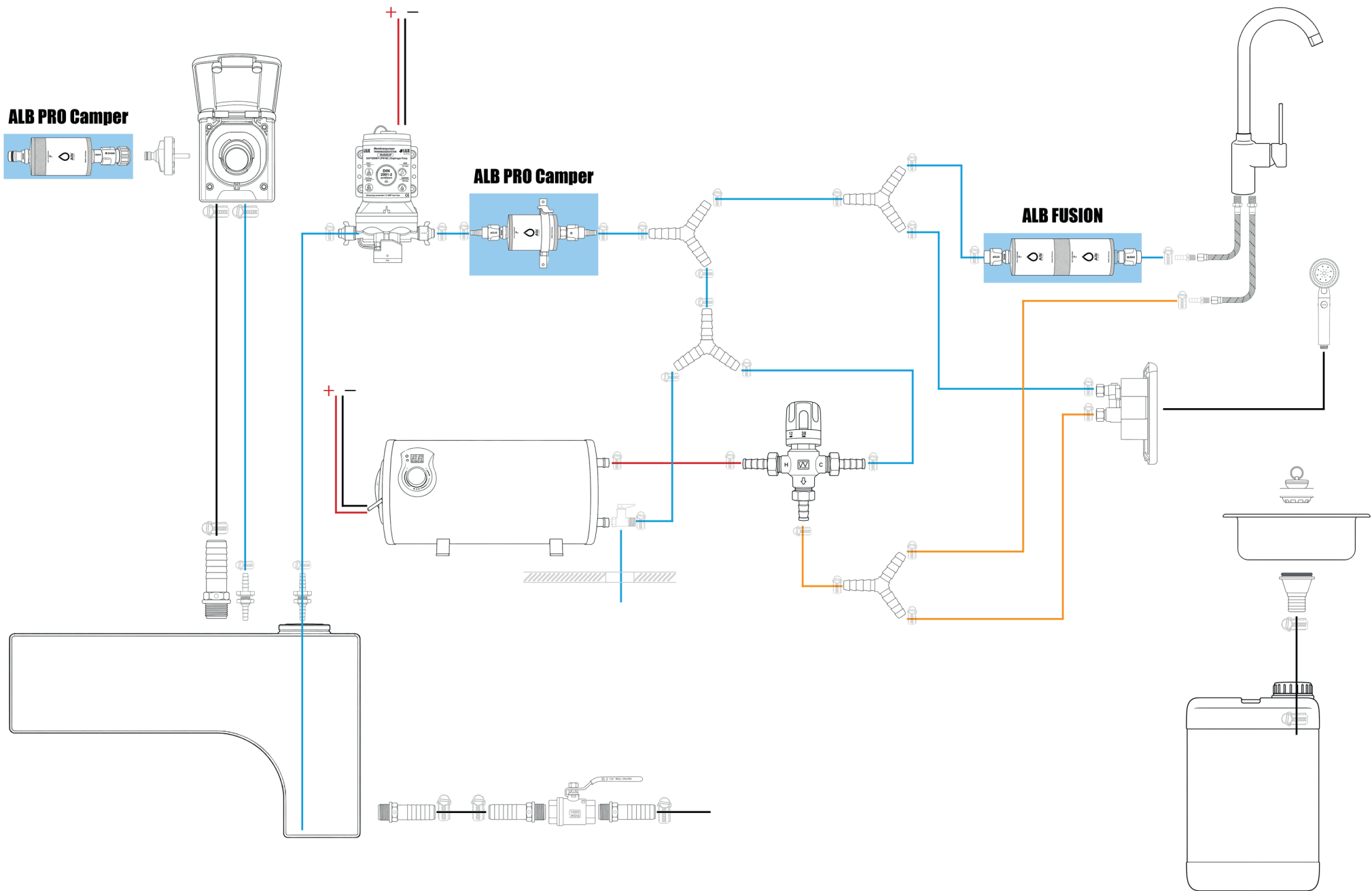
Schema Wasser (Boiler, Abwasserkanister, ALB)
